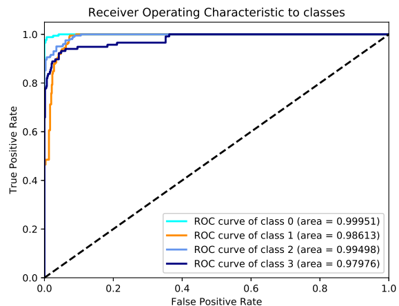
Fig. 7: Individual class ROC curves of mobile net on large scale image are shown. The classes 0-3 are clean, anode, connection and damage, respectively.
